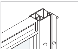
Without cover strip - chrome screw cover caps
